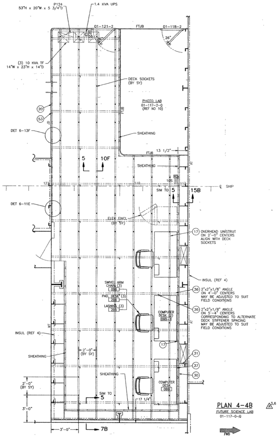
Figure 2: Existing Future Science Lab Floor Plan (420 WAGB 666-003)
