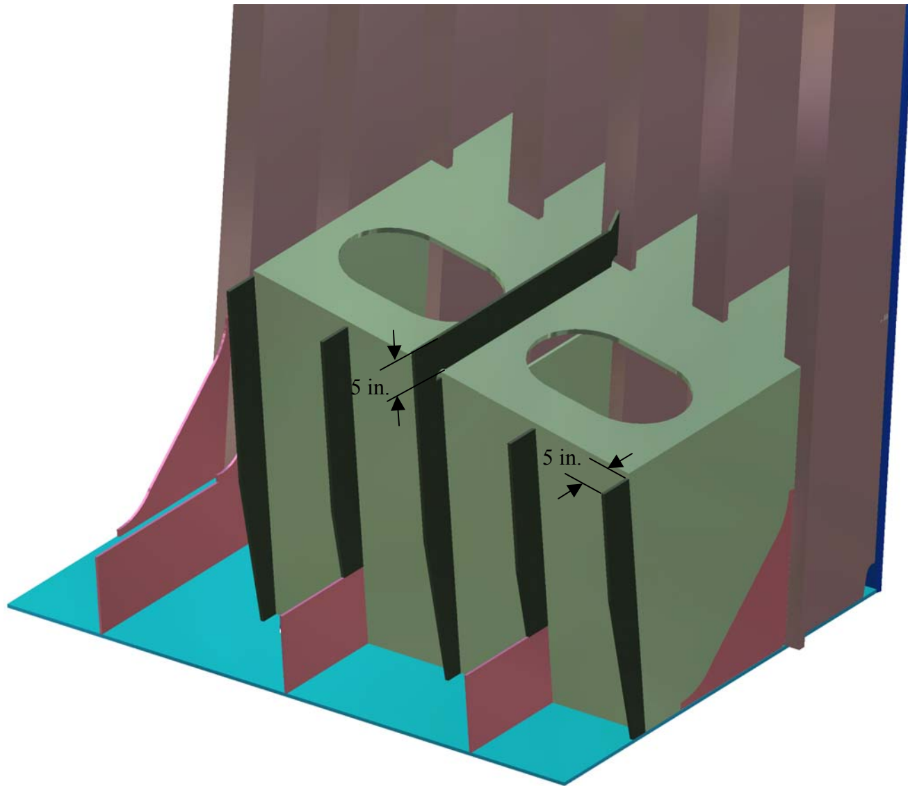
Figure 1c – Seachest with Access Hole Covers Off
