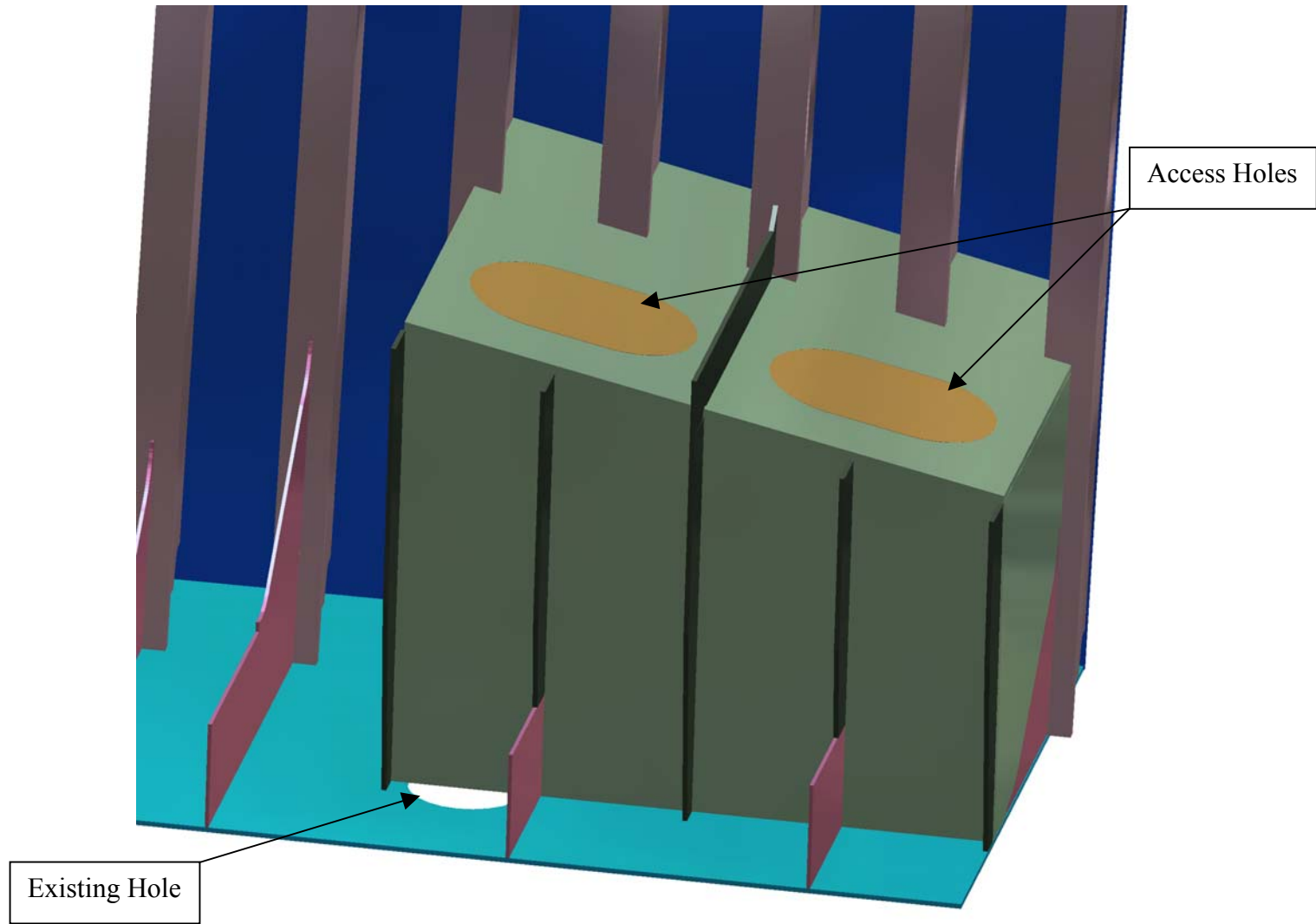
Figure 1b – Seachest with Access Hole Covers On
