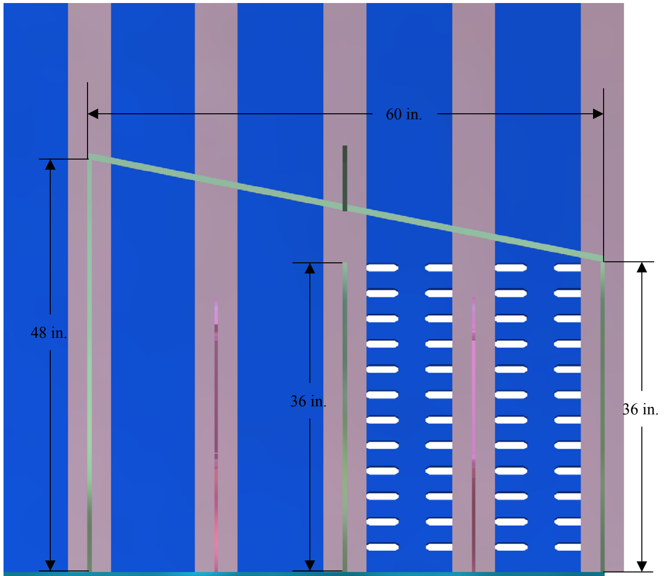
Figure 1f – Seachest Looking Outboard with Inboard Plate Removed
