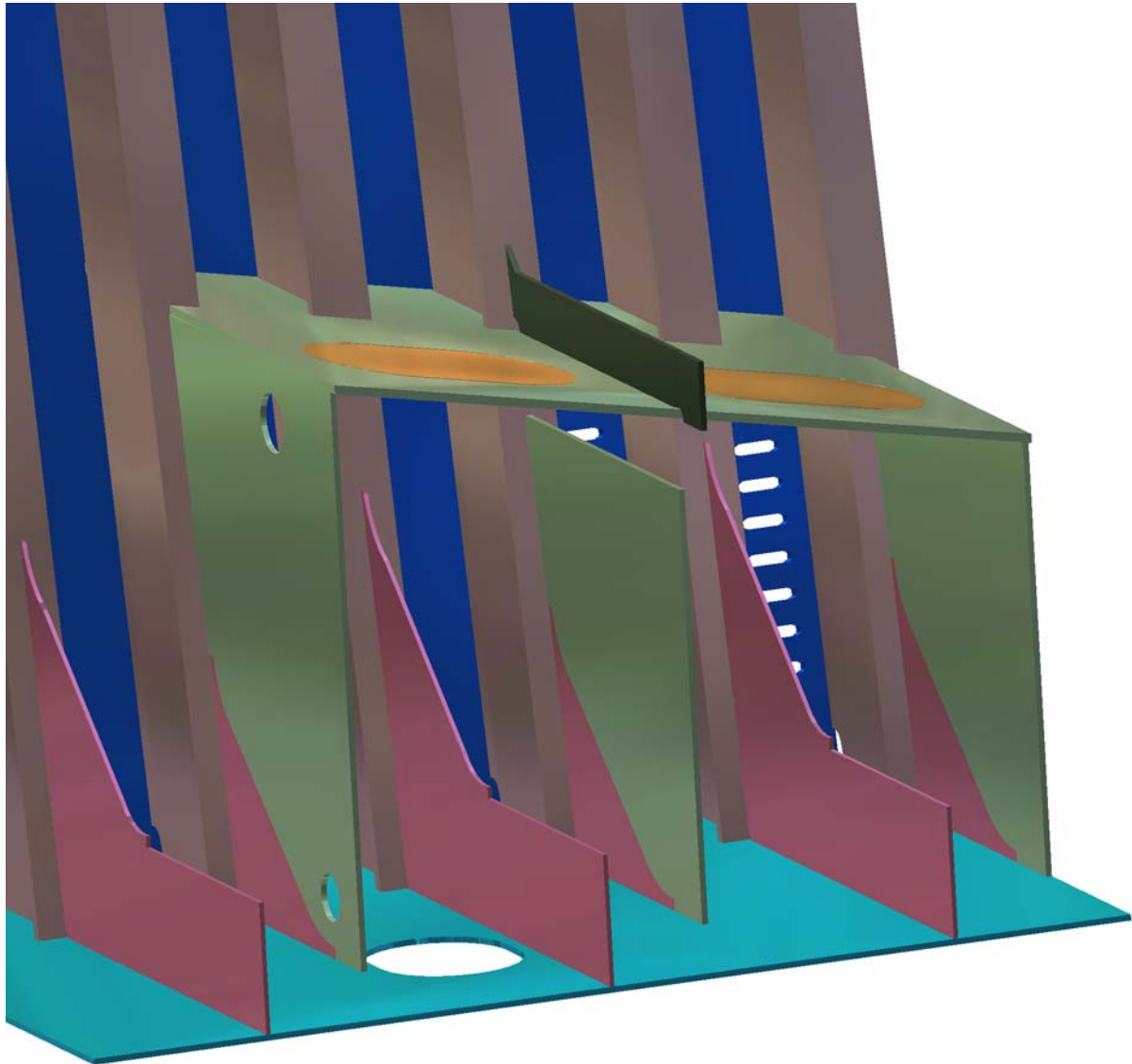
Figure 1d – Seachest Looking Outboard and Forward with Inboard Plate Removed
