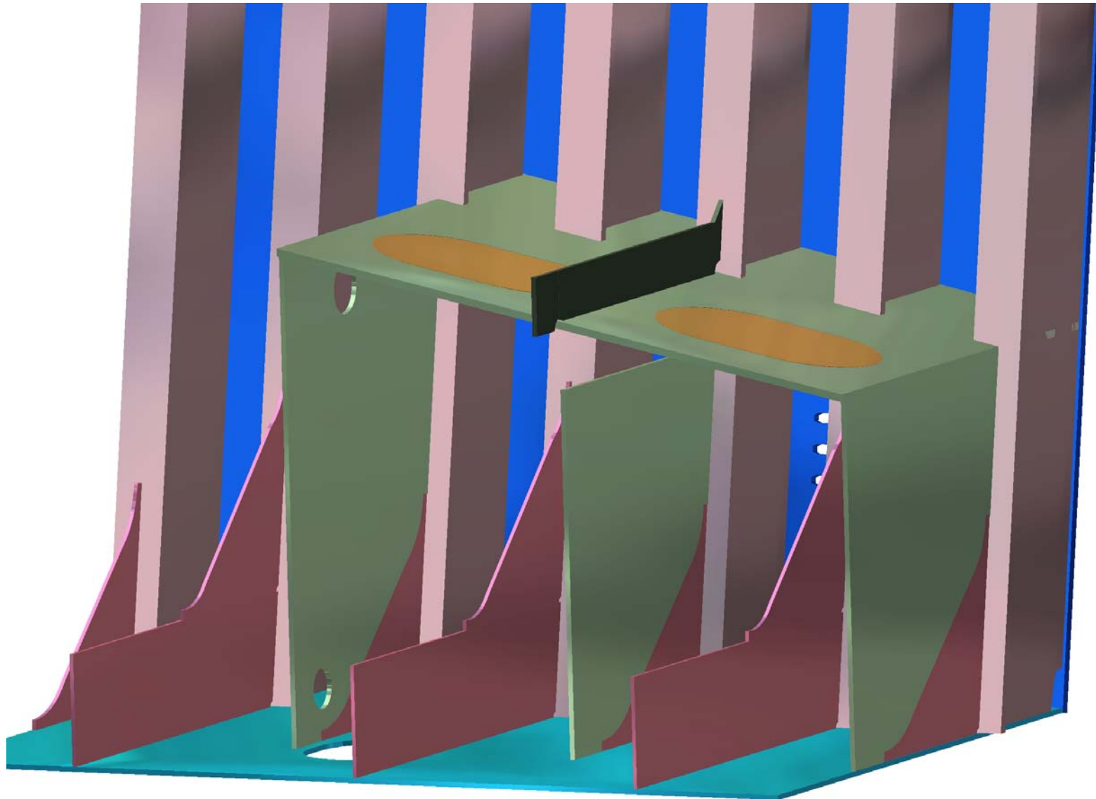
Figure 1e – Seachest Looking Outboard and Aft with Inboard Plate Removed
