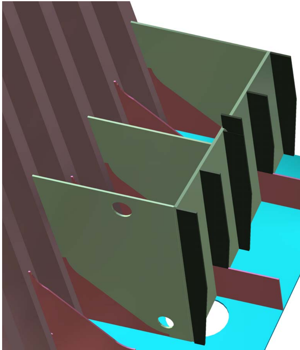
Figure 1j – Seachest Looking Forward and Down with Top Plate Removed
