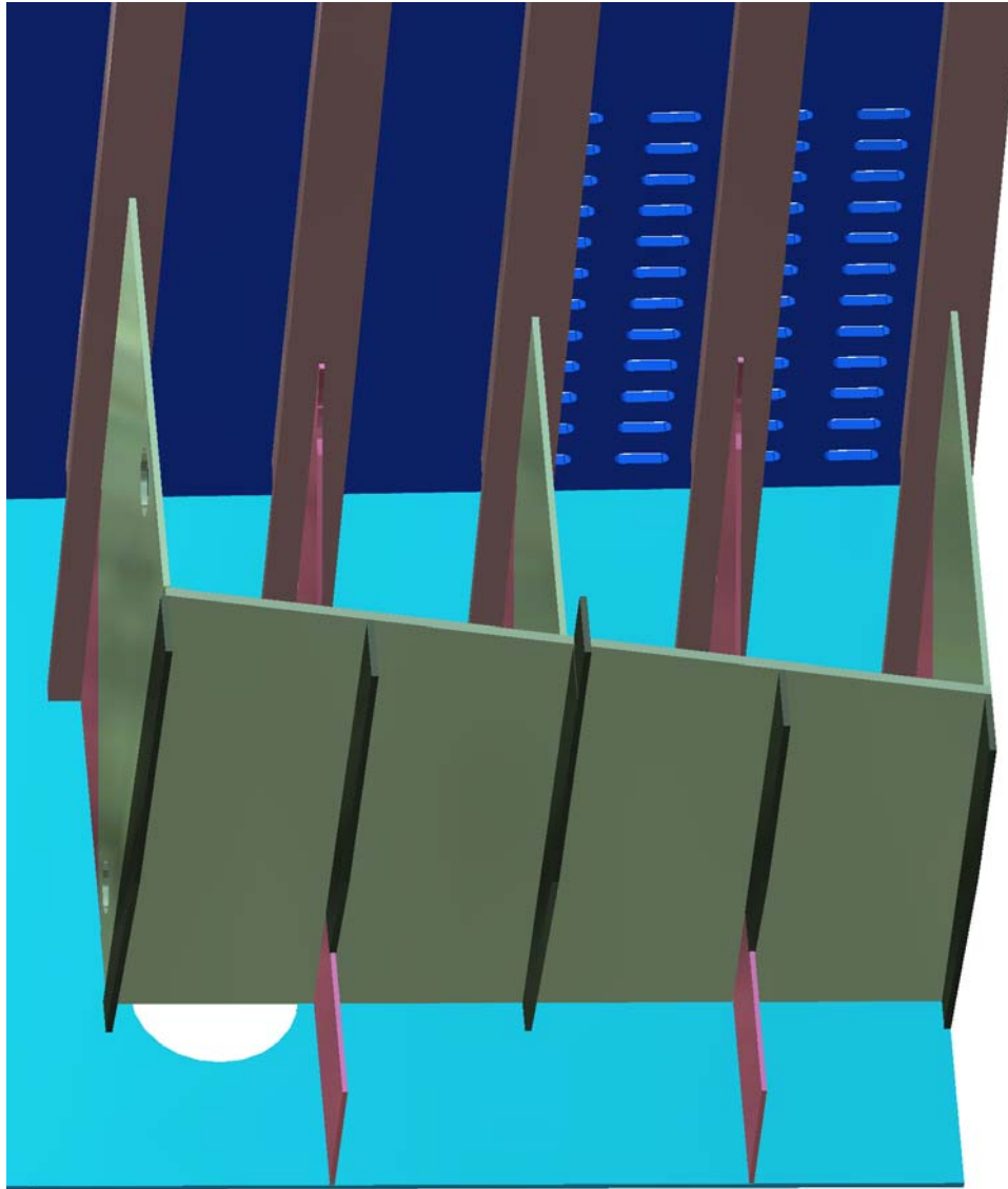
Figure 1g – Seachest Looking Outboard and Down with Top Plate Removed
