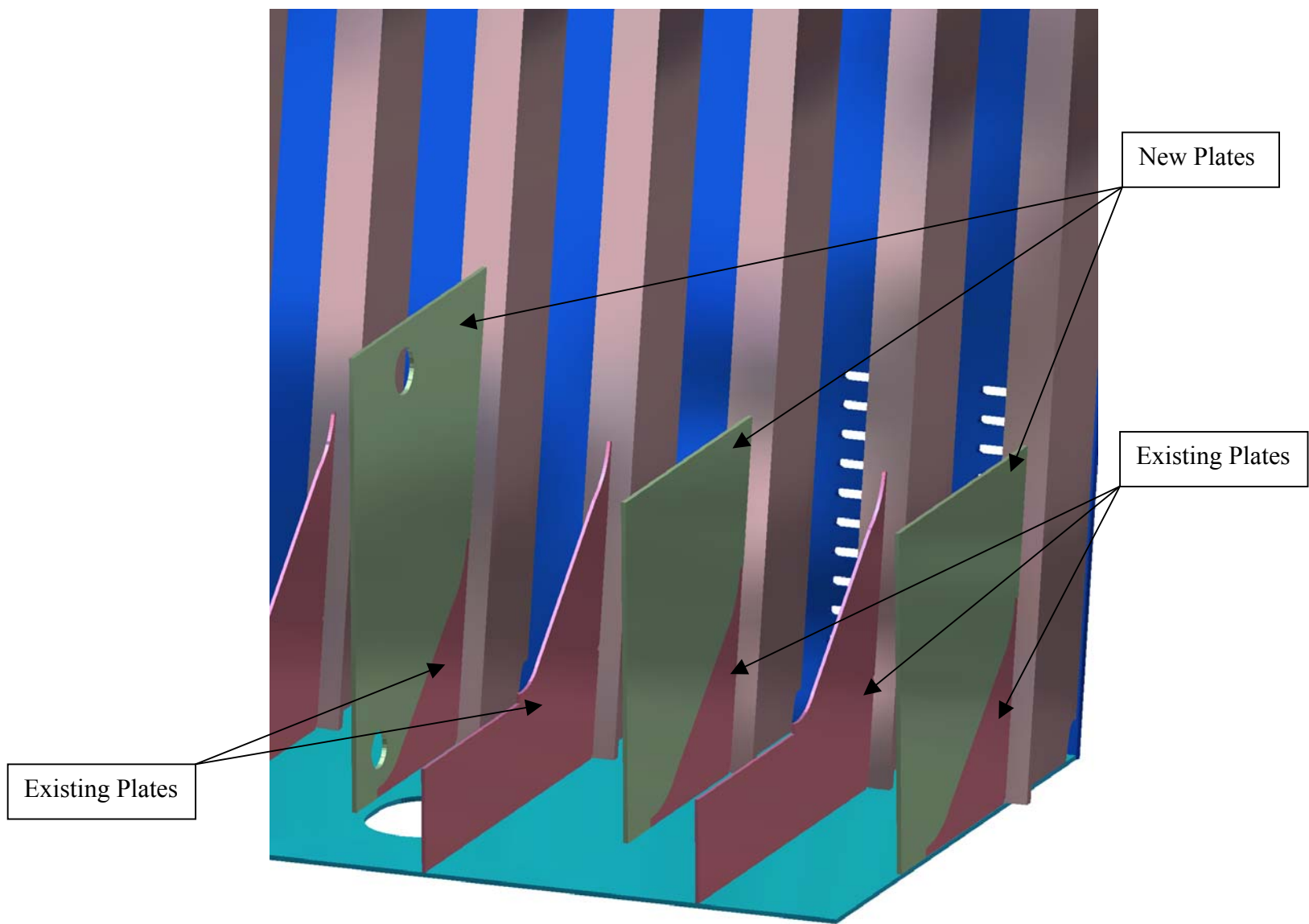
Figure 1k – Seachest with Top and Inboard Plates Removed
