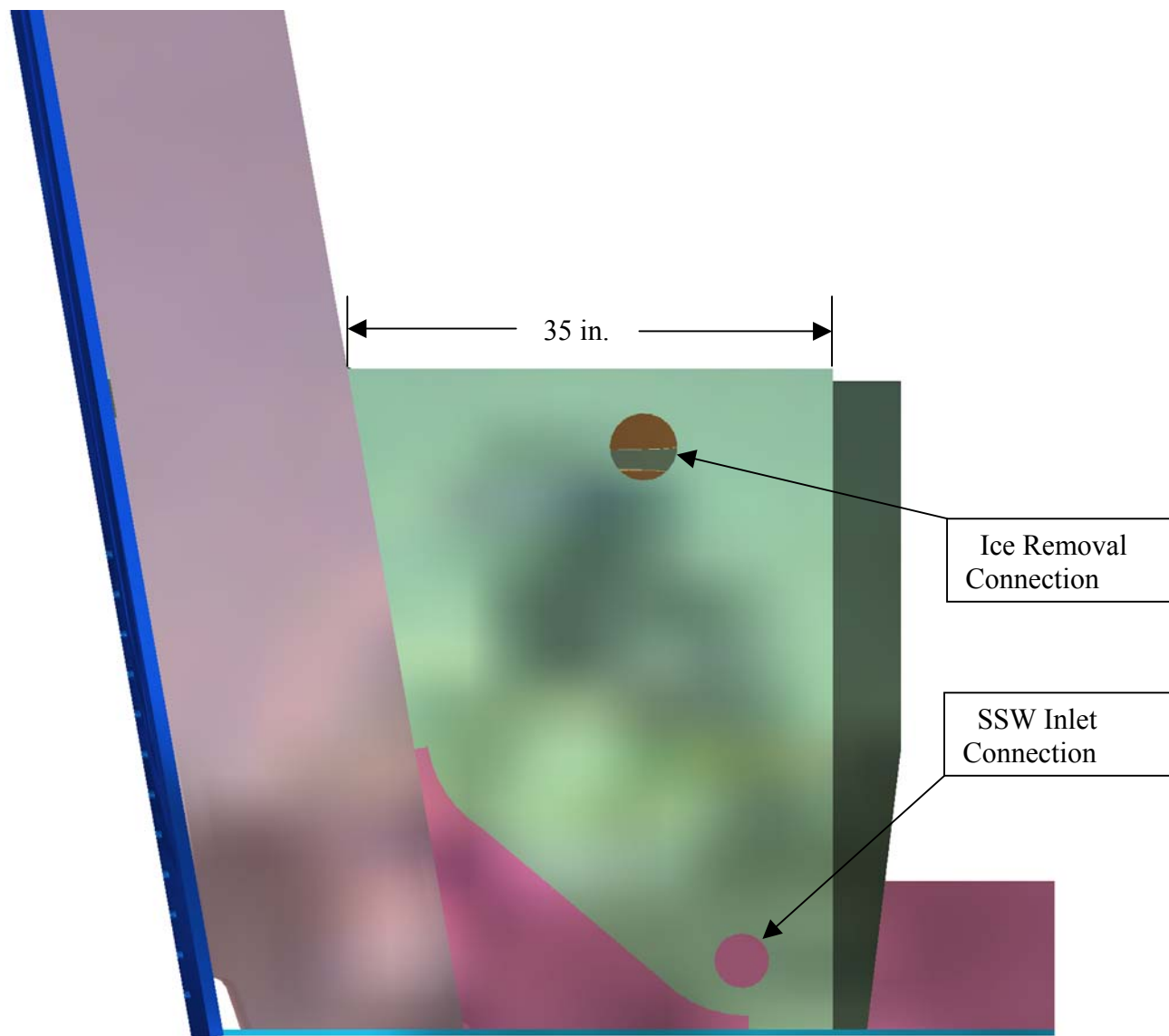
Figure 1i – Seachest Looking Forward
