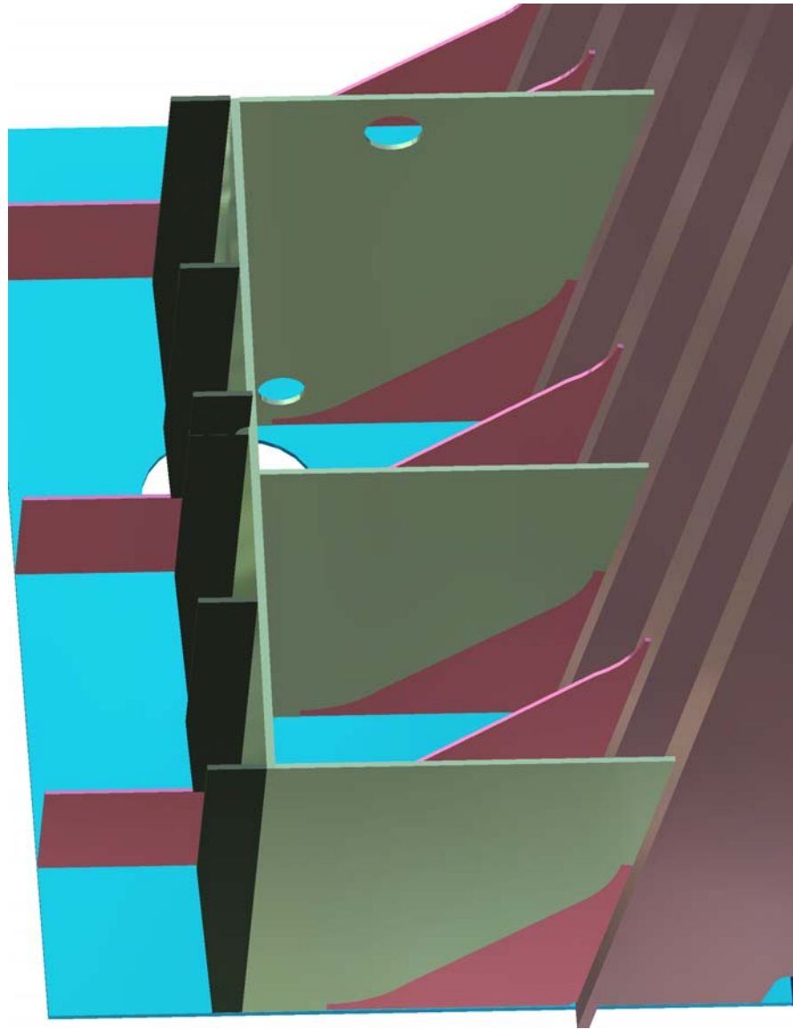
Figure 1h – Seachest Looking Aft and Down with Top Plate Removed
