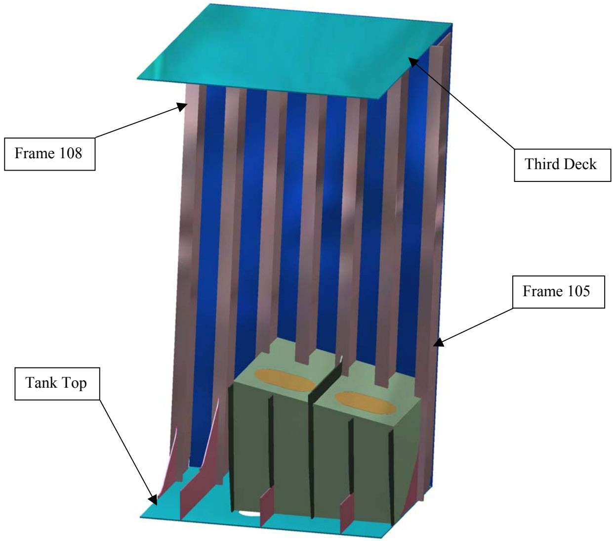
Figure 1a – Seachest Elevation View
