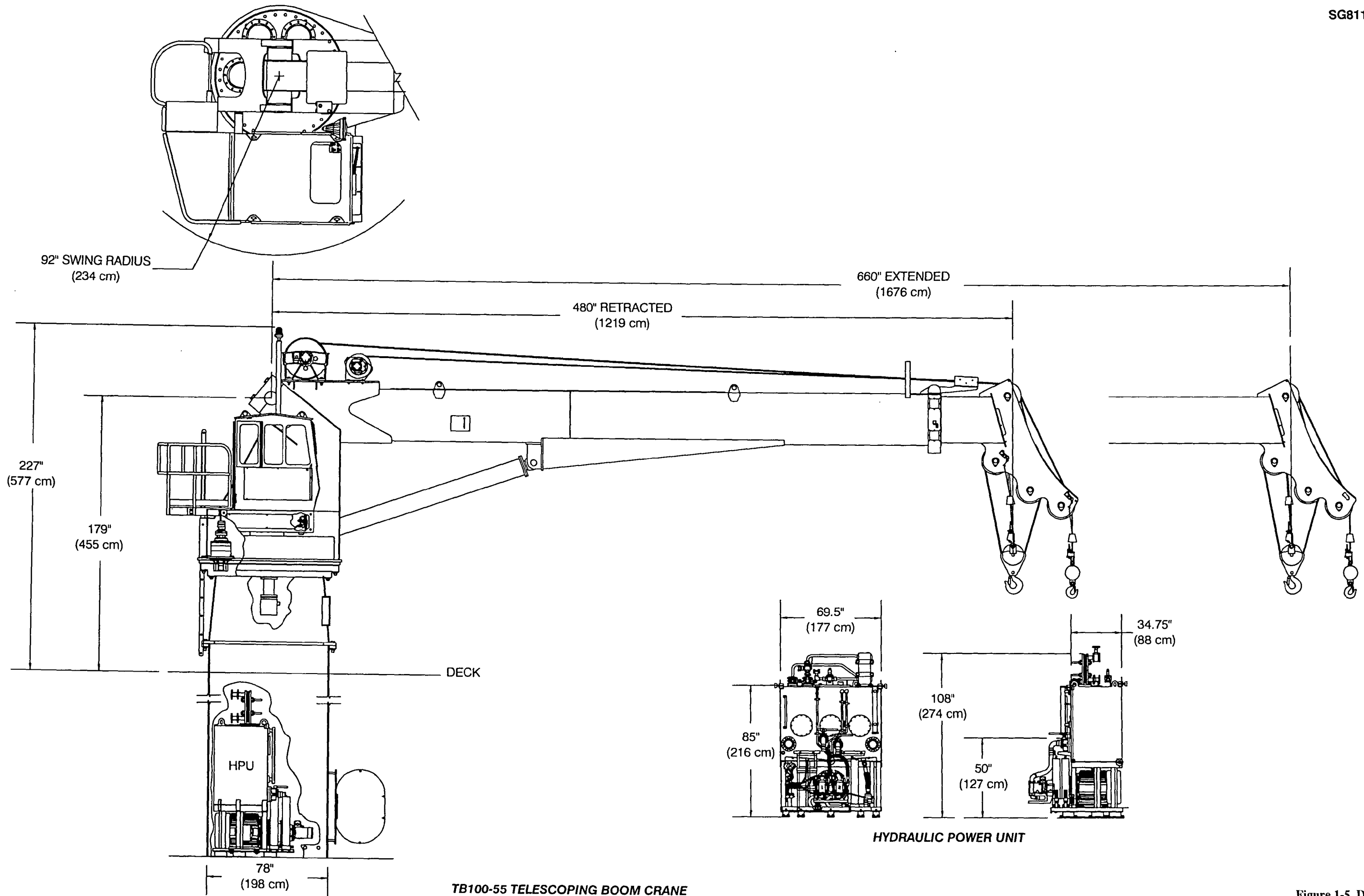
Figure 1-5 Dimensional Data
